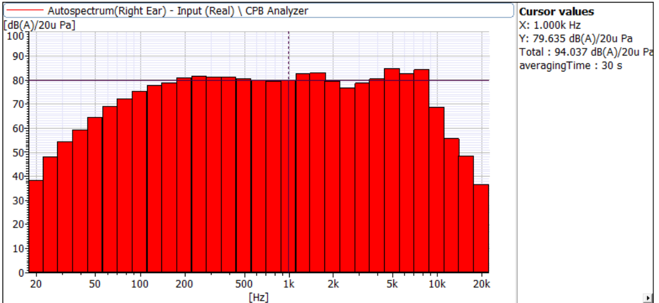
Figure 2: Representative picture indicates sound pressure level L_{Aeq} of Right ear reaches 94 dB(A) SPL. (Remark: 94 dB(A) SPL showed as a "Total" value in the figure is A-weighted equivalent continuous sound pressure level L_{Aeq} , use an averaging time of 30 seconds.)
